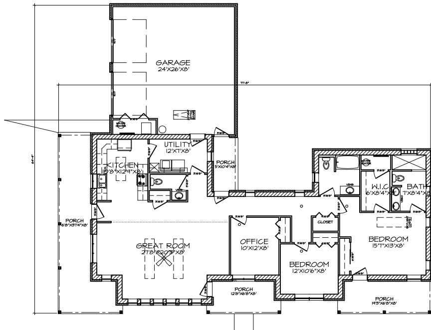
FIRST FLOOR PLAN A-4
