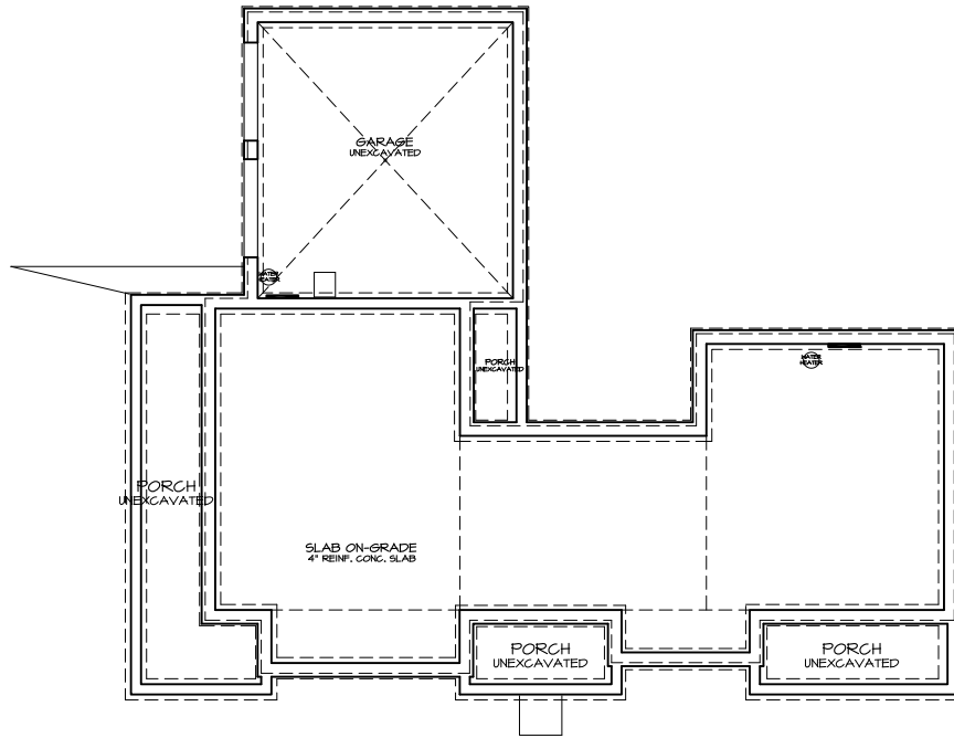
FOUNDATION PLAN A-3
